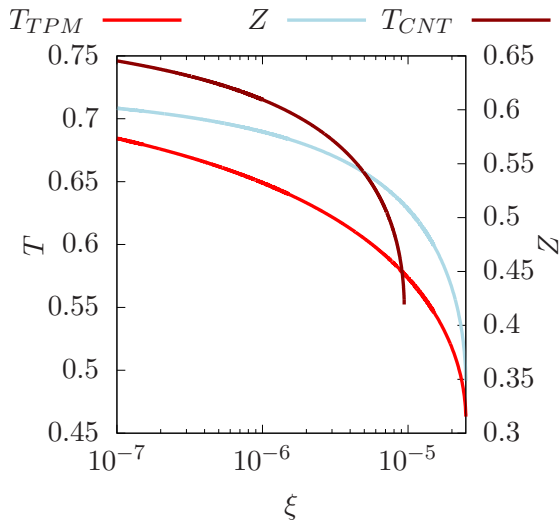
Рис. 6. Values of T and Z at t = t_{max}^S as functions of the cooling rate; n_{v0} = 3/130
