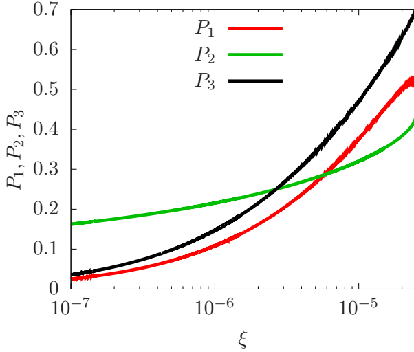
Рис. 9. Fulfillment of the validity criteria of the approximations used (32)–(34) at different cooling rates for n_{v0} = 3/130
