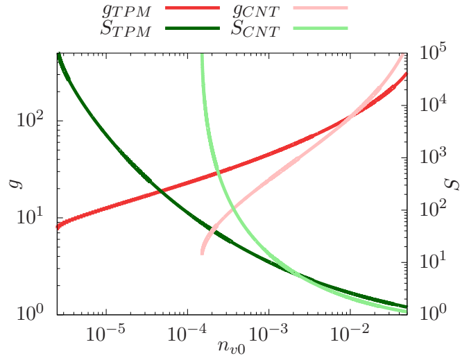
Рис. 7. Dependence of the critical size and the supersaturation on the total number density of particles at \xi = 10^{-10}
