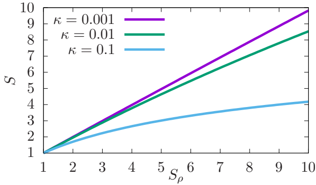
Рис. 2. Dependence of S on S_\rho for different \kappa
