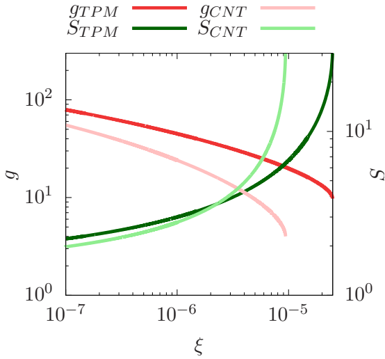
Рис. 5. Dependence of the critical size and the supersaturation on the cooling rate at t = t_{max}^S and n_{v0} = 3/130
