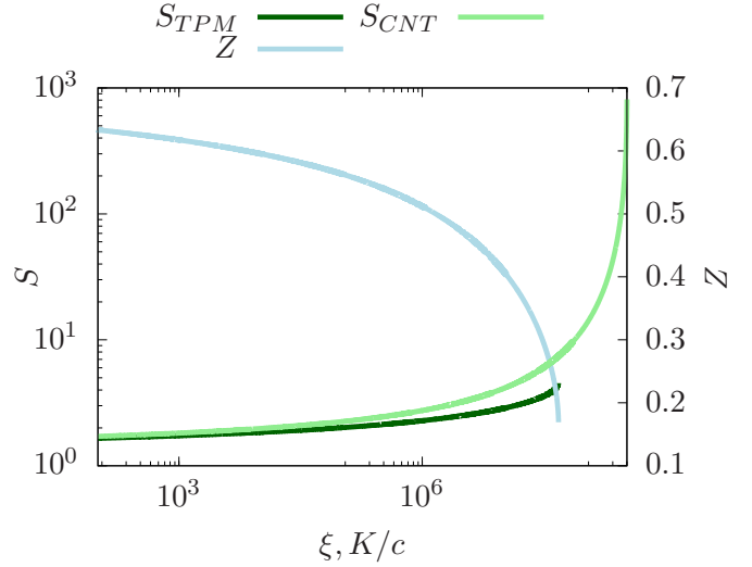
Рис. 13. Dependence of the supersaturation and the compressibility factor on the cooling rate \xi , calculated for the CNT and TPM models for the conditions [42]
