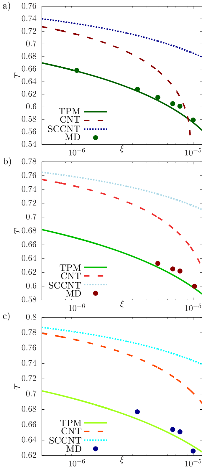
Рис. 10. Comparison of temperature at t = t_{max}^S as a function of \xi calculated using the analytical models CNT, SCCNT and TPM (curves) and obtained from MD simulation data (points) (see legend). a) n_{v0} = 3/130 , b) n_{v0} = 3.5/130 , c) n_{v0} = 4/130
