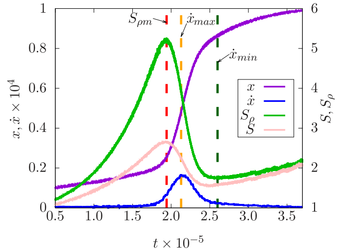
Рис. 3. Evolution of the main parameters of the system during MD simulation. \xi = 10^{-6} , n_{v0} = 3/130
