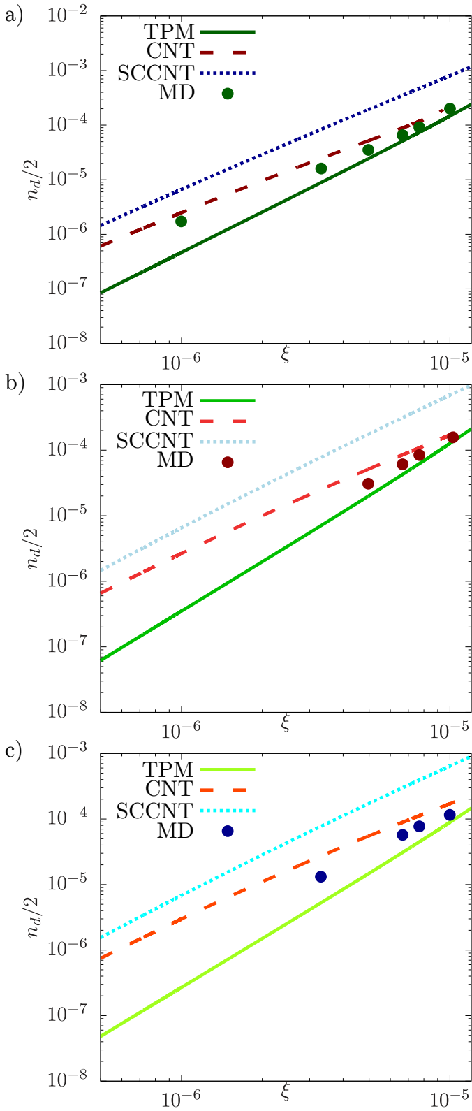
Рис. 12. Same as in Fig. 10, for the value n_d/2
