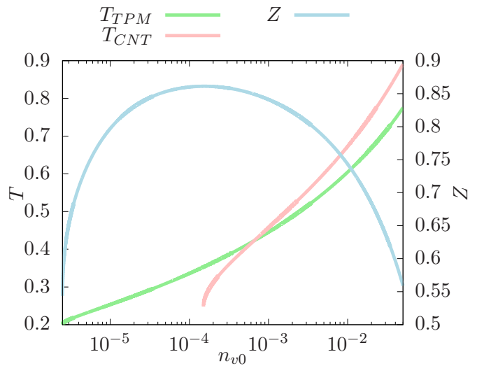
Рис. 8. Dependence of Z and T on the total number density of particles at \xi = 10^{-10}
