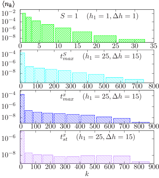
Рис. 4. Distribution of clusters over size n_k at times S = 1 , t_{max}^S , t_{max}^x and t_{st}^x (see the legend; the values of the parameters h_1 and \Delta h of the moving average (24) are given in brackets). \xi = 10^{-5} , n_{v0} = 3/130
