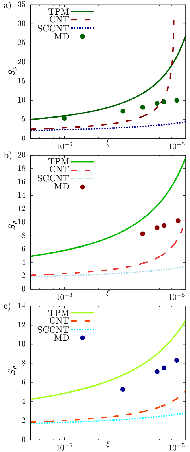
Рис. 11. Same as in Fig. 10, for the value S_p
