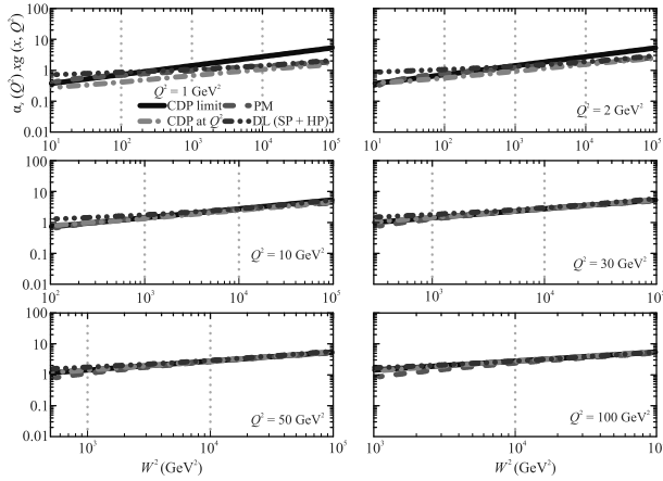
Fig. 1. (Color online) \alpha_s(Q^2)xg(x, Q^2) as a function of W^2 for various values of Q^2 in the CDP asymptotic limit (solid curve), PM (dashed curve) and soft-hard Pomeron model (SP + HP) (dashed-dot-dot curve)
