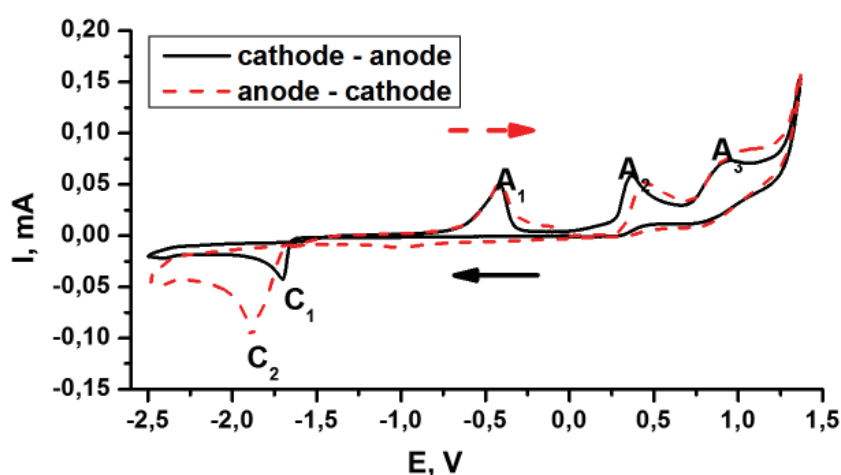
Fig. 5. CV curves of complex 12. Sweep of the working electrode potential from 0.00 V to -2.50 V, back to 0.00 V and then to 0.00 V (solid line); from 0.00 V to 1.40 V, then to -2.50 V and back to 0.00 V (dotted line).
