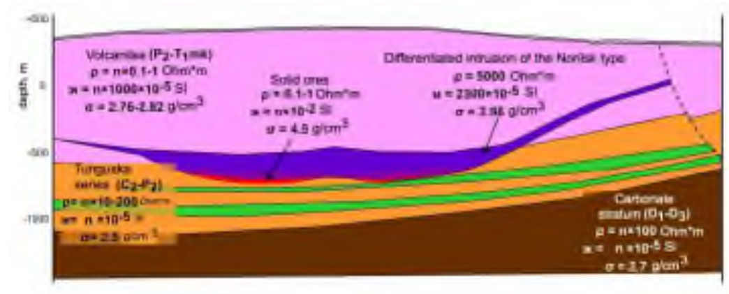
Figure 9. Generalized petrophysical model of the section that is typical for the Norilsk ore zone [Kulikov, 2017].
