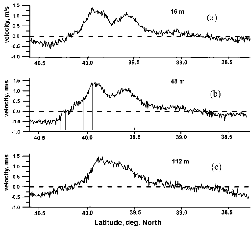
Figure 10. Characteristic variations in the longitudinal velocity (60°, east-northeast) of the Gulf Stream along the ship's route versus latitude at different depths in 2015. At depths of 16 m and 48 m, two current jets are seen, which merge deeper. Black vertical lines mark the intervals for assessing horizontal gradients.
