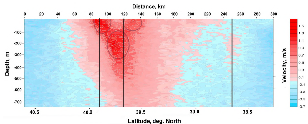
Figure 9. Cross-section of longitudinal (east-northeastern) component of velocity of the Gulfstream in 60^\circ direction on September 14, 2015. Positive values (rose) indicate downstream flow. The vertical lines indicate position of the profiles in Figure 11. Three cores of warm flow are outlined by ovals.
