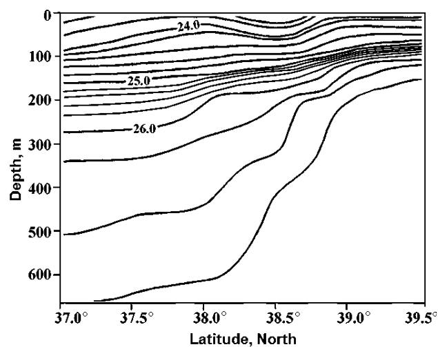
Figure 2. Section of density along 62°7' W based on the data of the first survey on September 20–22, 1989. Solid lines show isolines of density \sigma_T .
