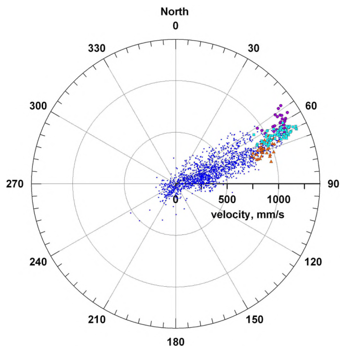
Figure 8. Polar diagram of the direction of currents measured by SADC during the crossing of the Gulf Stream region on September 14, 2015. Blue dots refer to the entire stream, purple circles to the upper northern core, orange triangles to the upper southern core, and turquoise squares to the lower core (in Figure 9).
