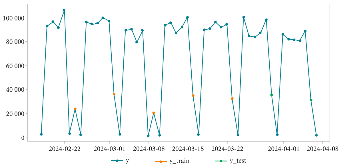
Fig. 14. Time series of weekdays
