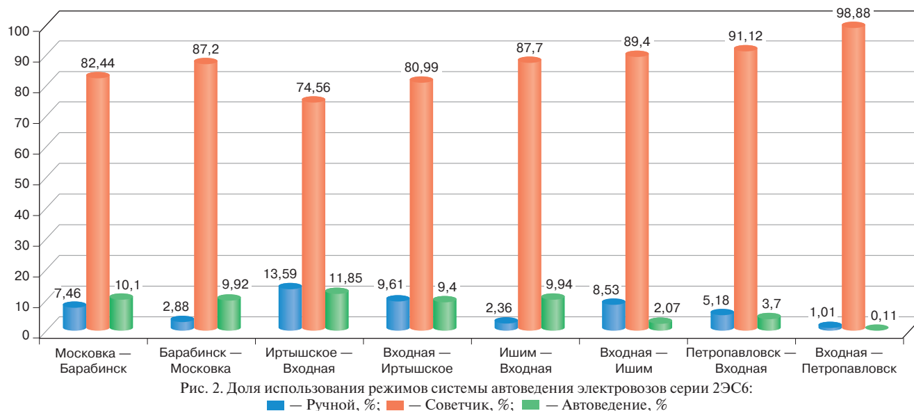
Fig. 2. Share of auto-driving system modes used on 2ES6 electric locomotives:
