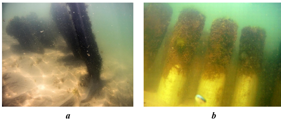
Fig. 4. State of the “Grebenska” breakwater modules: a – algae fouling and tilt of the structure (survey on 7 September 2022); b – post-storm partial exposure of the wave-damping piles from under sand (survey on April 12, 2023)
