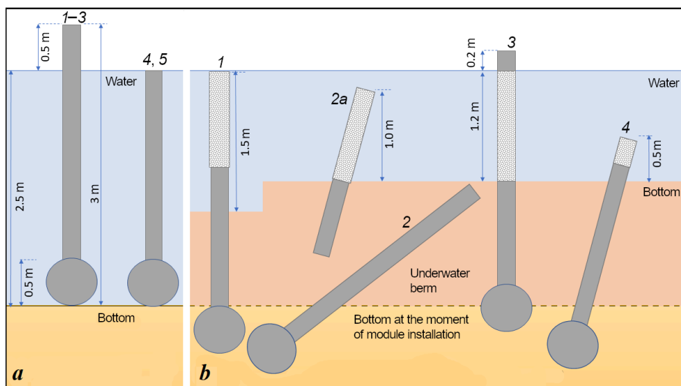
Fig. 5. Schematic initial position of the modules (1–5) during installation in May 2021 ( a ) and their final position during the survey on 07.09.2022 ( b ). The parts fouled with algae are highlighted in light gray. The diagram shows the subsidence of modules and their sanding up, deviations from the vertical axis, and changes in the height of the surface part
