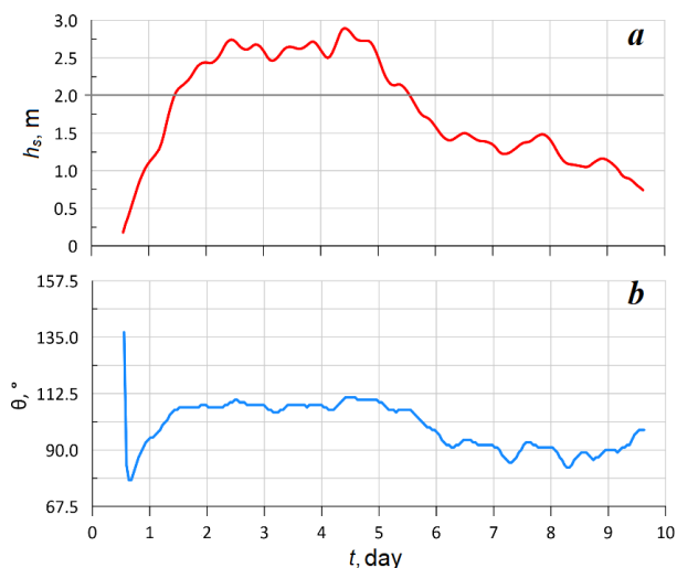
Fig. 5. Significant wave heights (a) and mean wave direction (b) in the central part of Koktebel Bay for storm (S3) which is extreme by duration ( T = 95 hours, h_s = 2.6 m, SPI = 625 \text{m}^2\cdot\text{h} ) according to SWAN-ERA data
