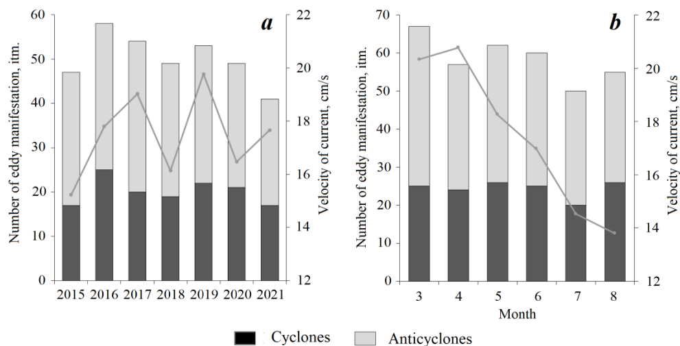
Fig. 3. Distribution of the number of mesoscale eddies and average velocity of currents (gray line) in the upper layer based on CMEMS reanalysis data by years ( a ) and months ( b )
