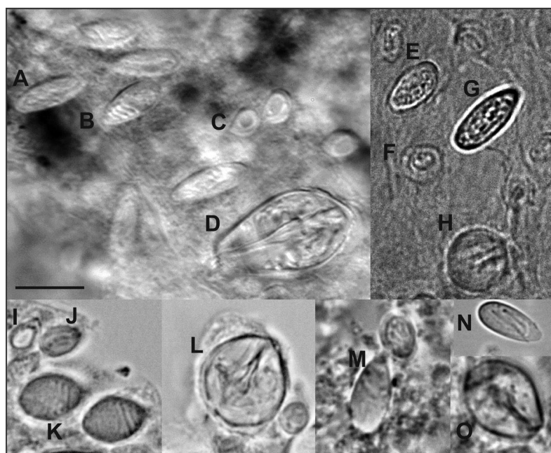
Fig. 2. Nematocysts of different Hydra species: A–D – H. oxycnida ; E–H – H. oligactis ; I–L – H. circumcincta ; M–O – H. vulgaris . A, E, J, N – atrichous isorhizas; C, F, I – desmonemes; B, G, K, M – holotrichous isorhizas; D, H, L, O – stenoteles. Scale bar is 10 \mu m.
