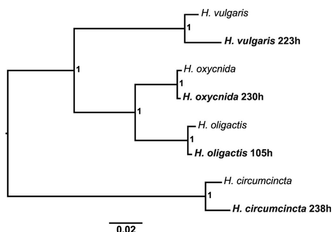
Fig. 3. Combined COI and ITS1–5.8S–ITS2 phylogenetic tree. Haplotypes of hydras from the Baikal region are in bold
