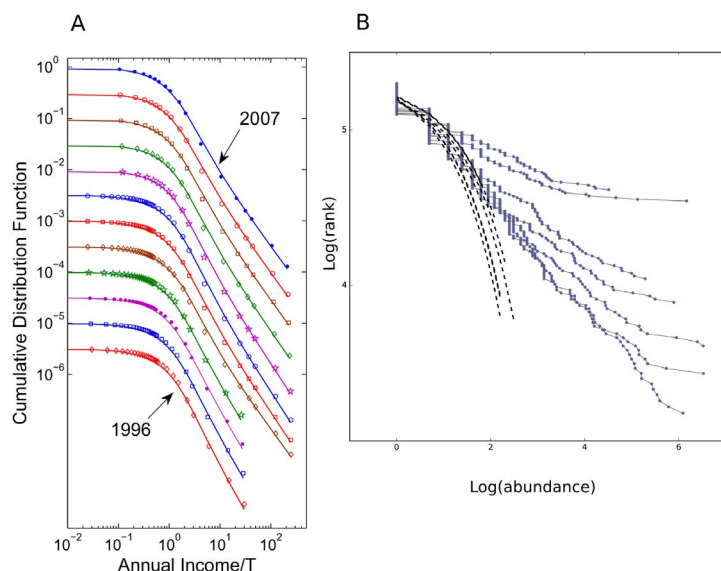
Fig. 3. Cases of dependencies where a description combined from power-law and exponential models could be applied.
