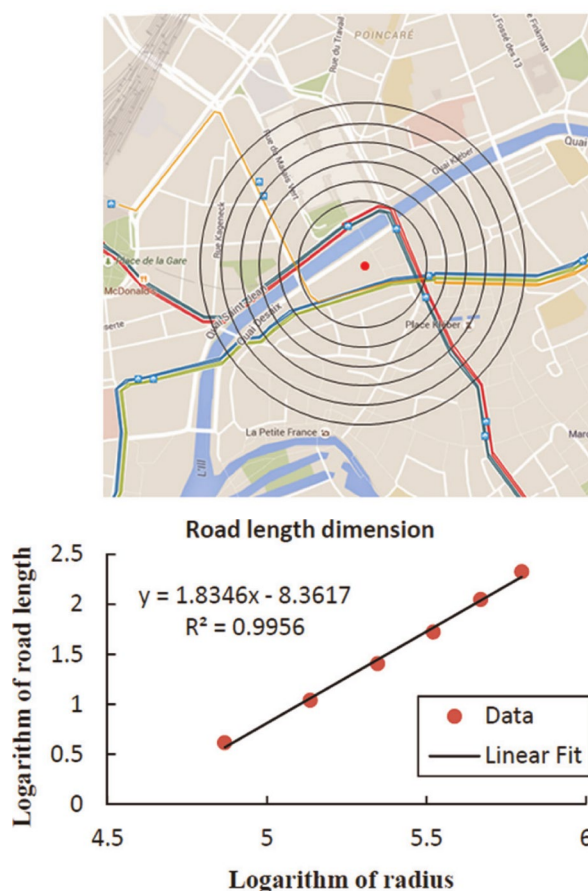
Fig. 2. Detection of fractal structure for the road network in Strasbourg, France. Adopted from (Wang et al., 2017)
