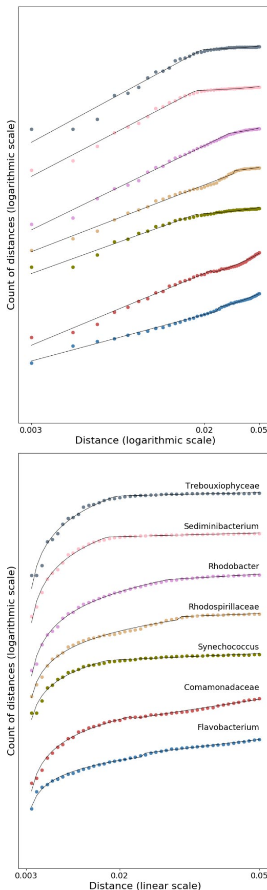
Fig. 5. The distributions of paired distances between fragments obtained by the sequencing of the V4-V6 region of the 16S rRNA genes. The distributions for fragments which have identity > 95\% to the reference annotated sequences are shown for 7 selected genera. The same distributions are shown in both parts of the chart, at different scales.
