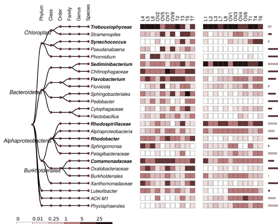
Fig. 4. A composition of microbiomes for healthy and diseased sponges, for the 25 most abundant genera of bacteria and chloroplast. Bars on the right show the significance of difference in abundances between healthy and diseased samples, for each genera. Collection sites are notated as follows: L - Listvyanka, OV - Olkhon Gate, T - Turali cape.
