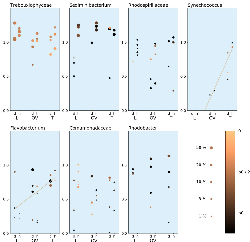
Fig. 7. Values of fractal dimension (Pareto coefficient) and a coefficient in the Boltzmann-Gibbs part of distance-based distributions for selected genera, estimated in separated samples. The separate samples are shown as circles in each part of the chart. The slope of the first part of the distribution (the fractal dimension part), defines the Y-coordinate of each sample. The size of the circle reflects the relative abundance of the selected genus in the microbial community, and color notations are used to show the slope of the regression line in the second part of the distributions (a coefficient for the Boltzmann-Gibbs model). The X axis is used to separate the places of collection and the disease states of the samples. The scales for sample size and for the Boltzmann-Gibbs coefficient are shown at the bottom right of the chart. The values for the Boltzmann-Gibbs coefficient are scaled separately for each part of the chart, relatively to reference value b_0 specific for each genera and listed in Table 2.
