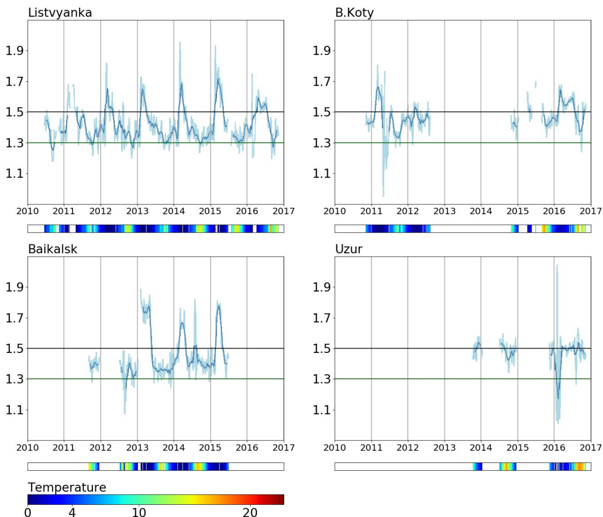
Fig. 8. The fractal dimension calculated for fluctuations of water temperature, in four locations in Lake Baikal. The fractal dimension (Y axis) was calculated at 16-hour intervals, using the Higuchi approach. The X axis shows the dates of measurement. The color bars at the bottom part of each subplot directly show the measured values of temperature. A light-blue line directly shows an estimated time dependency of the Higuchi dimension, and a dark blue line shows the same dependency smoothed using moving average with window size equal to 50 data points.
