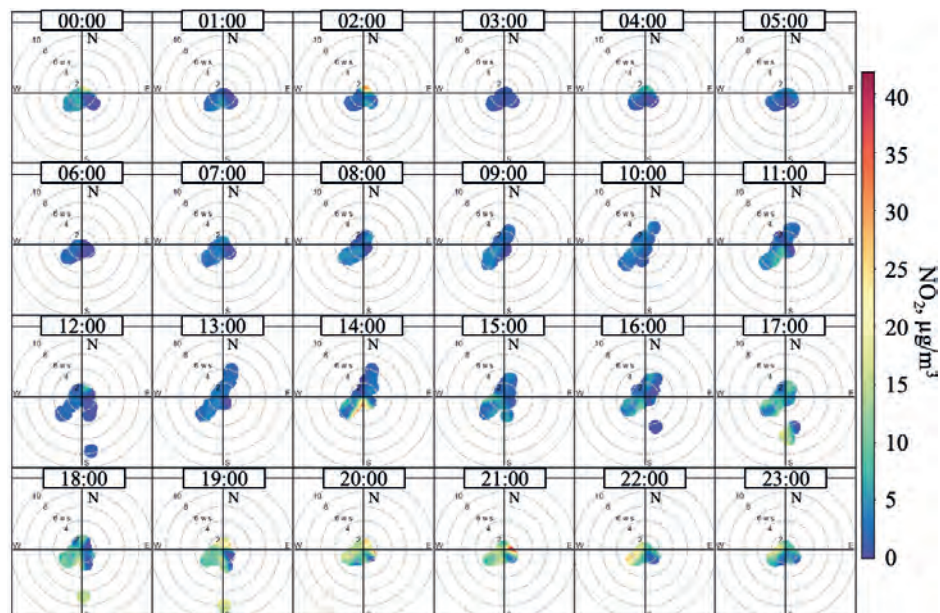
Fig.7. NWR analysis for ten-minute concentrations of \text{NO}_2 in the polar coordinate system at the «Boyarsky» station, July 2023.
