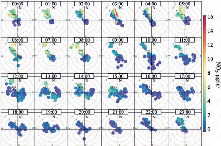
Fig.4. NWR analysis for ten-minute concentrations of NO 2 in the polar coordinate system at «Listvyanka» station, July 2023.
