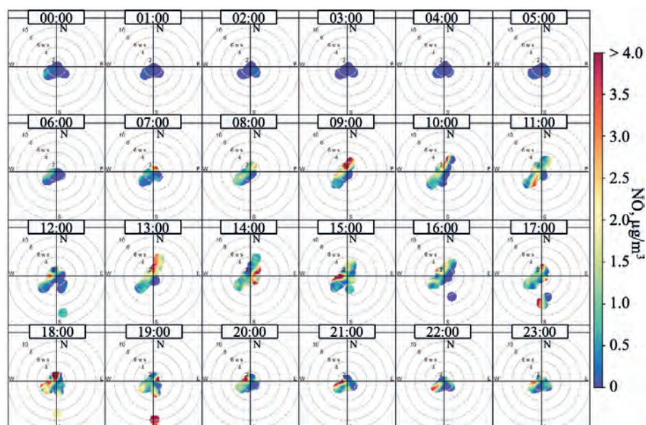
Fig.8. NWR analysis for ten-minute concentrations of \text{NO} in the polar coordinate system at the «Boyarsky» station, July 2023.
