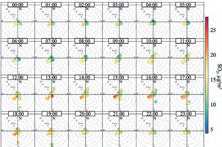
Fig.6. NWR analysis for ten-minute concentrations of SO 2 in the polar coordinate system at the «Boyarsky» station, July 2023.
