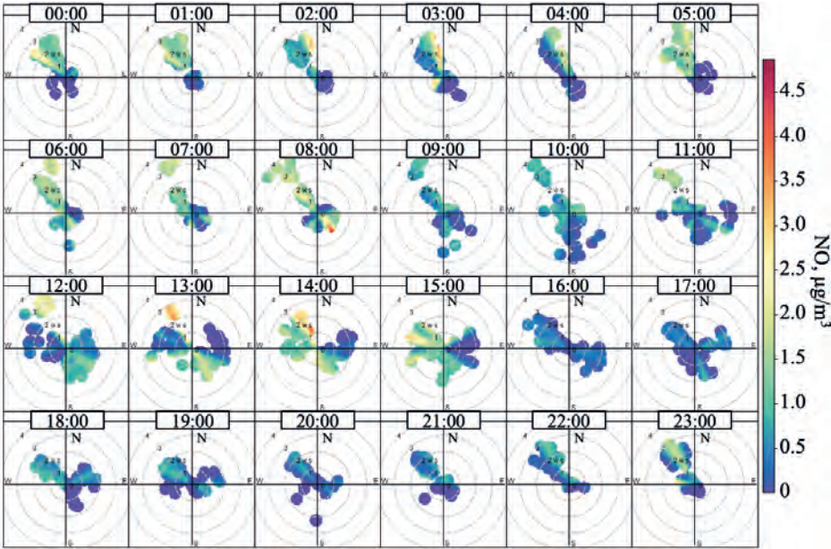
Fig.5. NWR analysis for ten-minute concentrations of NO in the polar coordinate system at «Listvyanka» station, July 2023.
